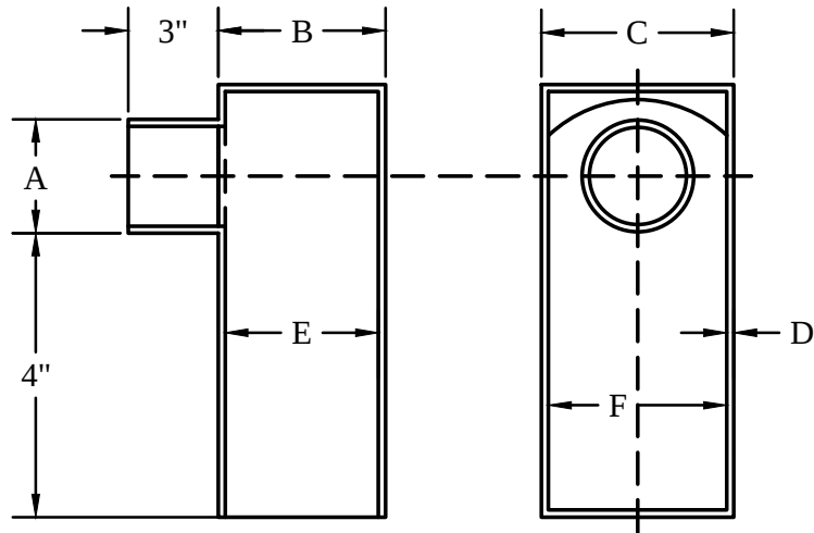
90° ADAPTER DETAIL
